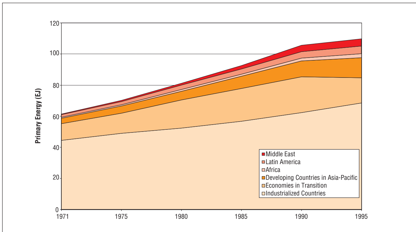
Figure 3.4: Primary energy use in the buildings sector, 1971-1995.
