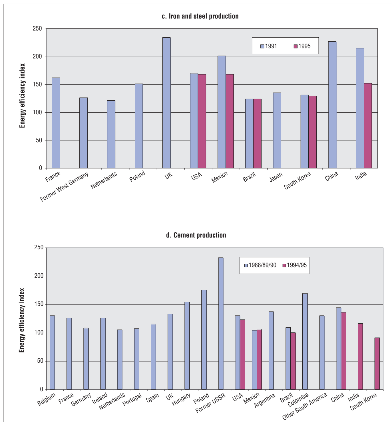
Figure 3.13c - d: Relative levels of energy efficiency for selected industrial sectors in various countries. The aggregate energy efficiency index (EEI) is calculated as:
