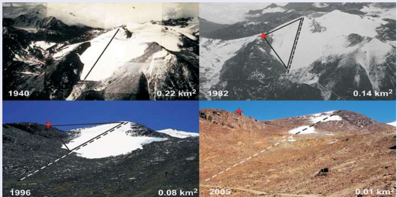
Figure 5.10: Areal extent of Chacaltaya Glacier, Bolivia, from 1940 to 2005. By 2005, the glacier had separated into three distinct small bodies. The position of the ski hut, which did not exist in 1940, is indicated with a red cross. The ski lift had a length of about 800 m in 1940 and about 600 m in 1996 (shown by a continuous line in 1940 and a broken line in all other panels) and was normally installed during the precipitation season. After 2004, skiing was no longer possible. Photo credits: Francou and Vincent (2006) and Jordan (1991). [WGII Figure 1.1]
